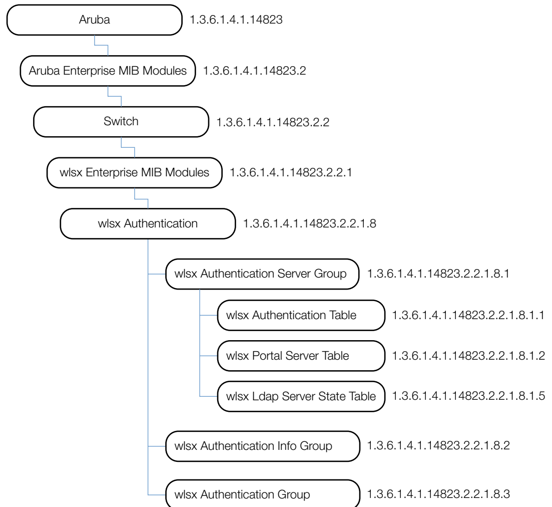
Figure 6 Authorization Hierarchy
